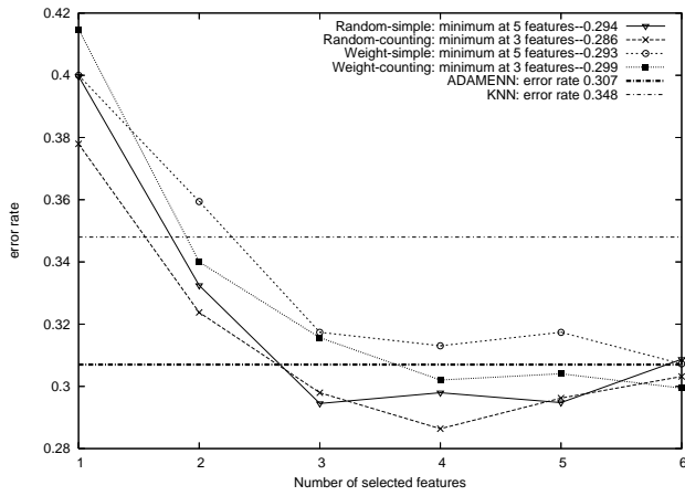
Figure 1: Liver data: Error rate as a function of the number of selected features for Random and Weight-driven methods.
