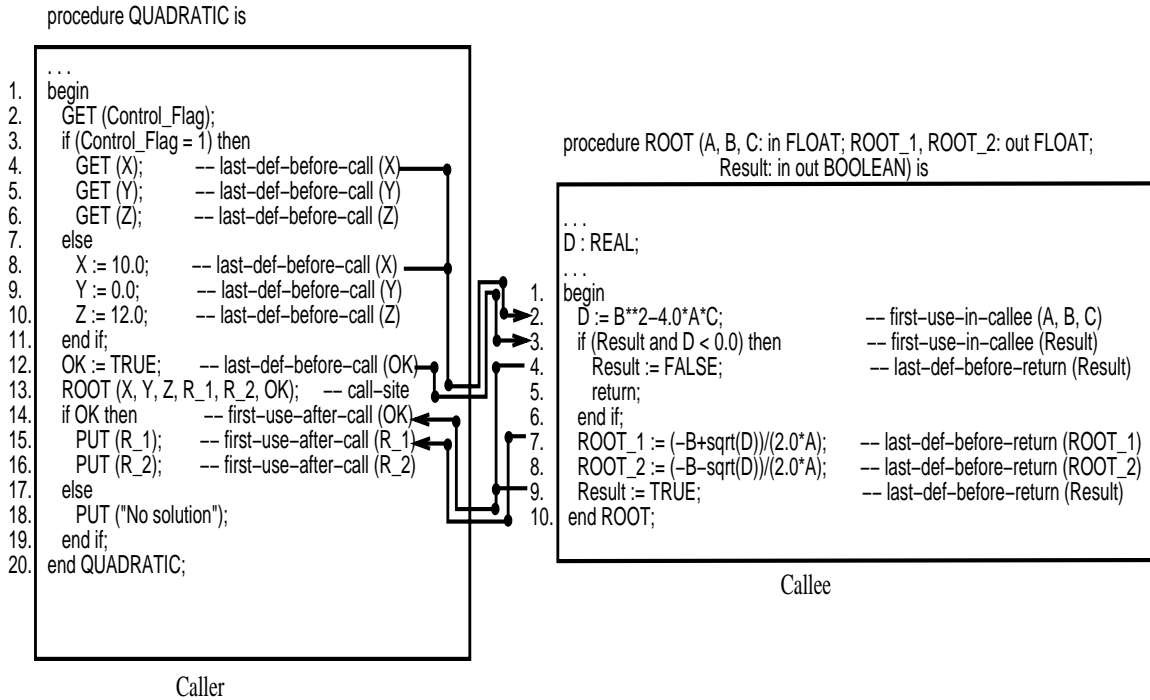
Figure 4: First Example of Coupling Paths
