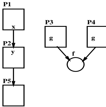
Figure 1: Example Call Graphs for Definitions
