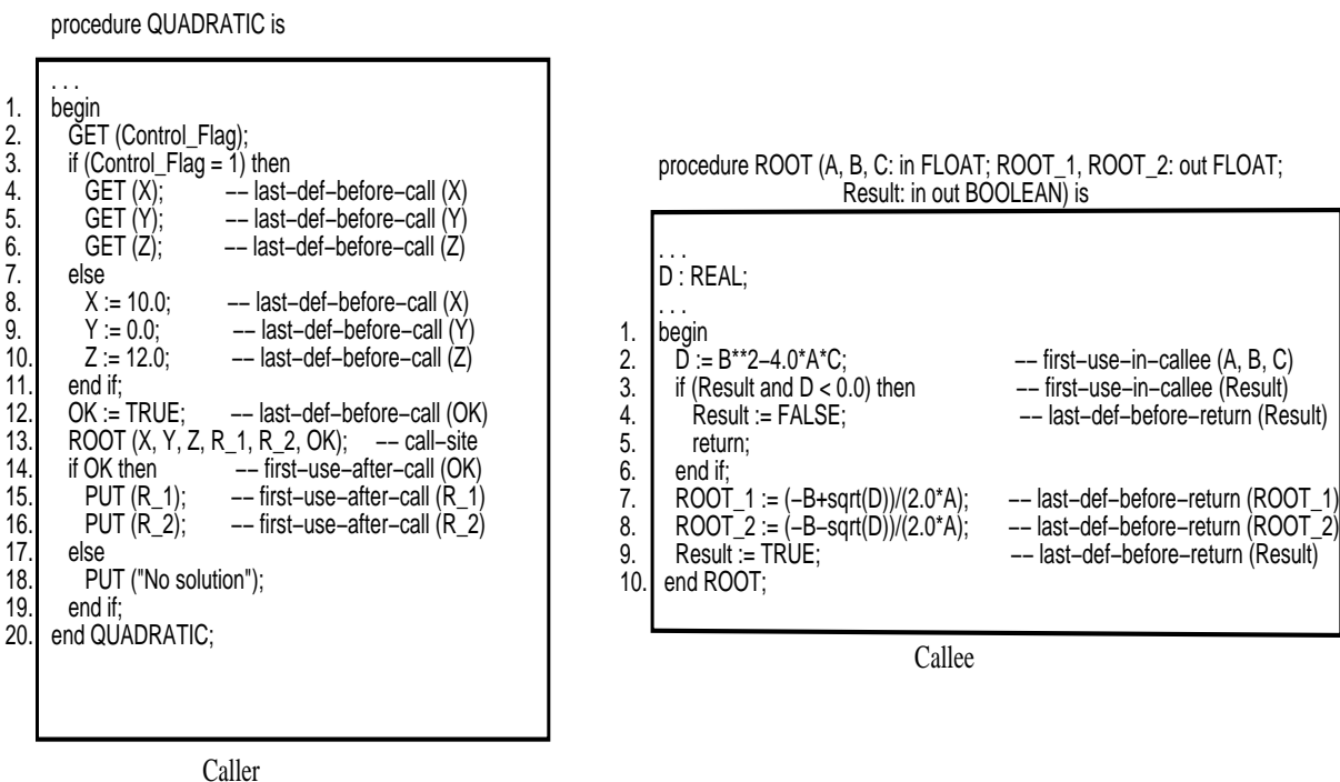
Figure 2: An Example of Coupling-uses and Coupling-defs
