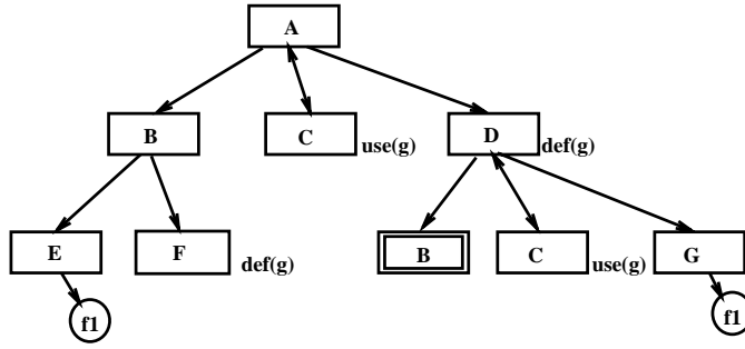
Figure 7: An Example of Coupling Graph
