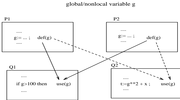
Figure 5: Second Example of Coupling Path
