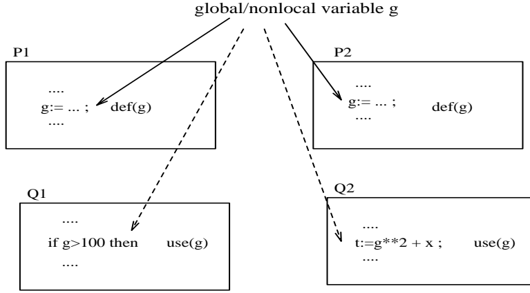
Figure 3: An Example of Shared-data Defs and Uses
